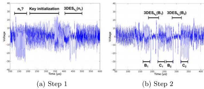
Fig. 4. Annotated traces during the authentication protocol (after analog processing)
