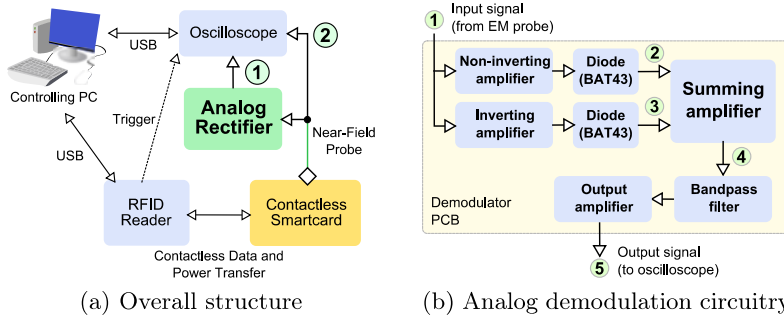
Fig. 1. Measurement setup
